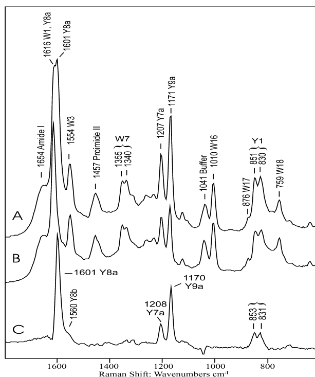
Fig. 3. 244 nm UVRR spectra of apohTf at (A) pH 6.25 and (B) 8.75. C: Difference spectrum of A minus B showing tyrosinate UVRR bands only, with minor features due to changes in buffer species.
